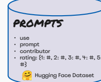
Prompts Dataset
